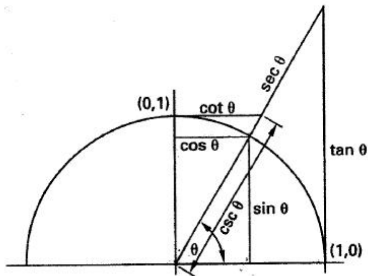
Figure 4.10 Trigonometric Functions in a Unit Circle
